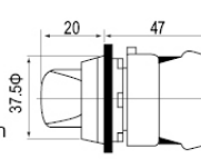
短柄带灯旋钮 Short shank with lamp knob
