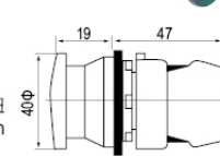
大头带灯按钮 Big head with lamp button
