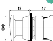
急停按钮 Emergency stop button
