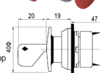
急停钥匙旋钮 Emergency stop key knob
