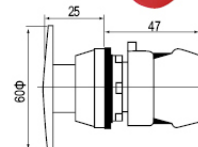
急停按钮 Emergency stop button
