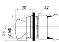
长柄带灯旋钮 Long handle with lamp knob
