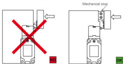
The actuator must not strike directly against the switch head.
